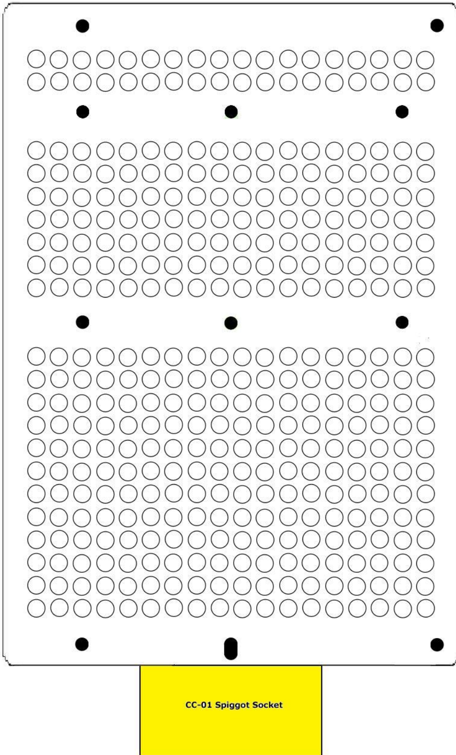
Figure 4 CA-01 level 2 top view 3mm thick plate
