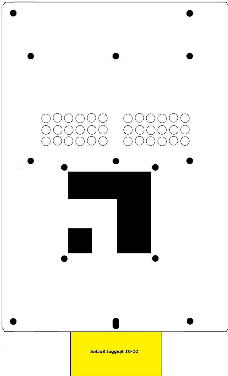
Figure 7 CA-01R level 2 underside view 3mm plate
