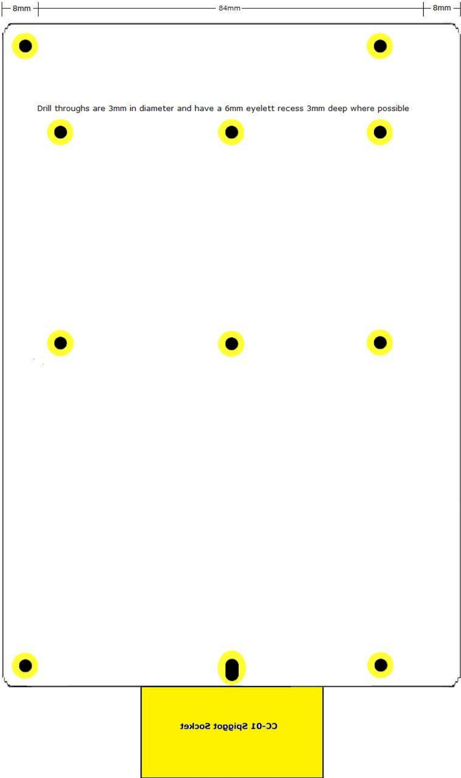
Figure 2b underside view of CA-01 level 1
