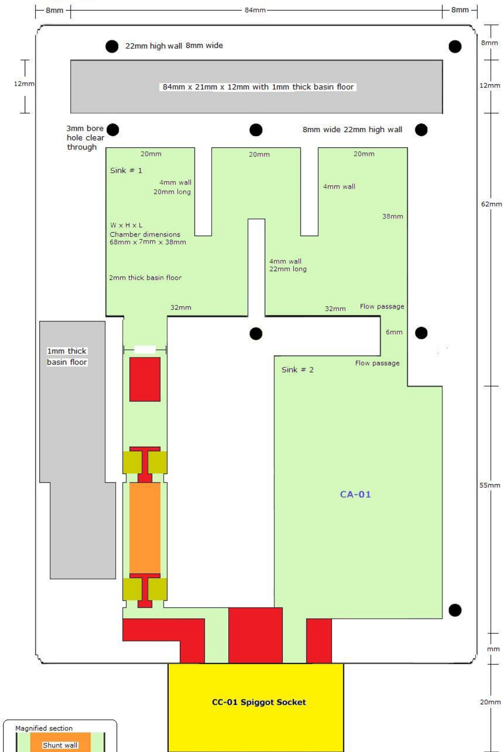
Figure 1 chamber dimensions level 1 Flat underside
