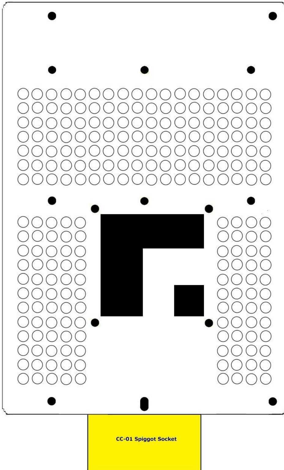
Figure 6 CA-01R level 2 top view 3mm thick plate
