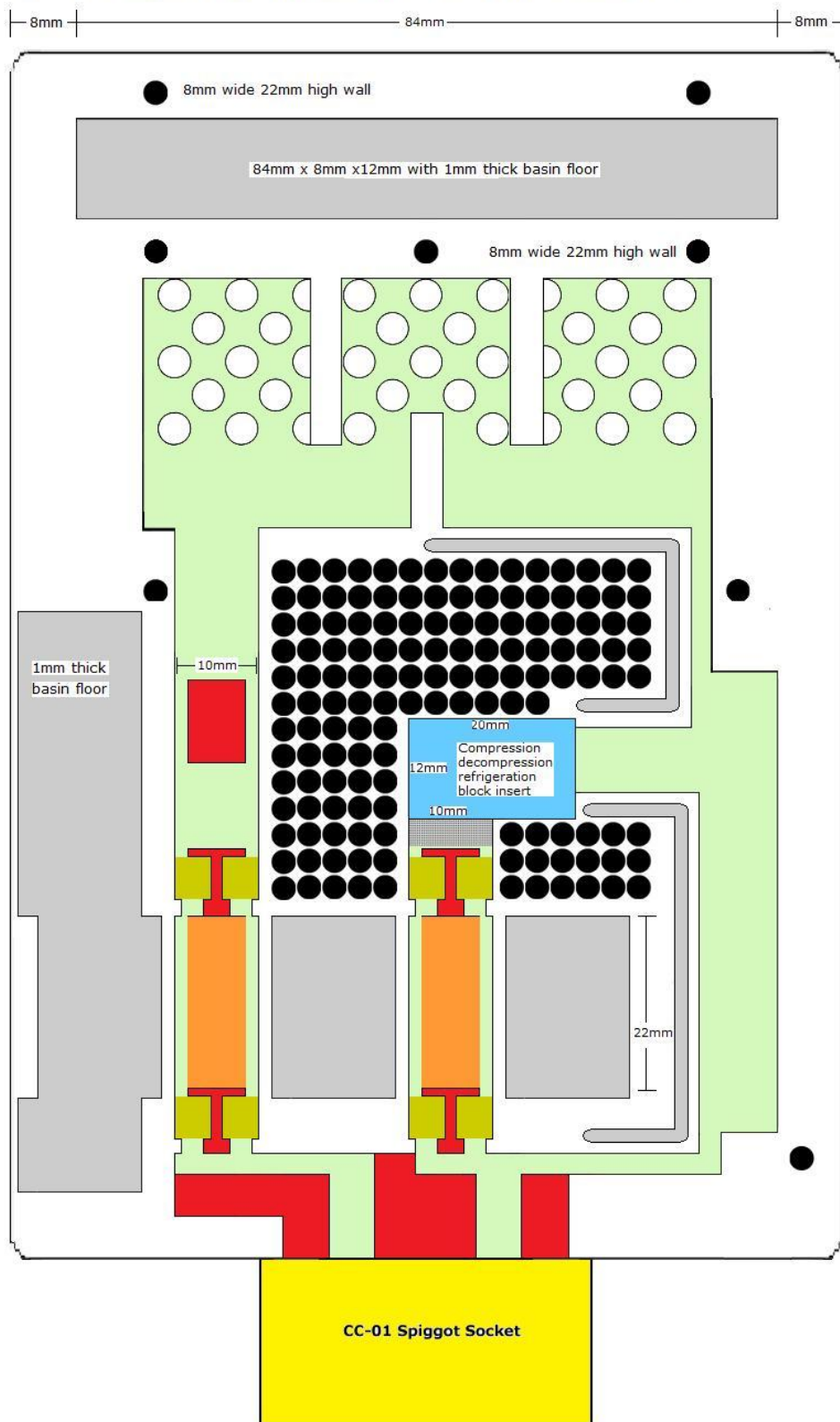
Figure 3 chamber dimensions level 1 CA-01R : Refrigerate
